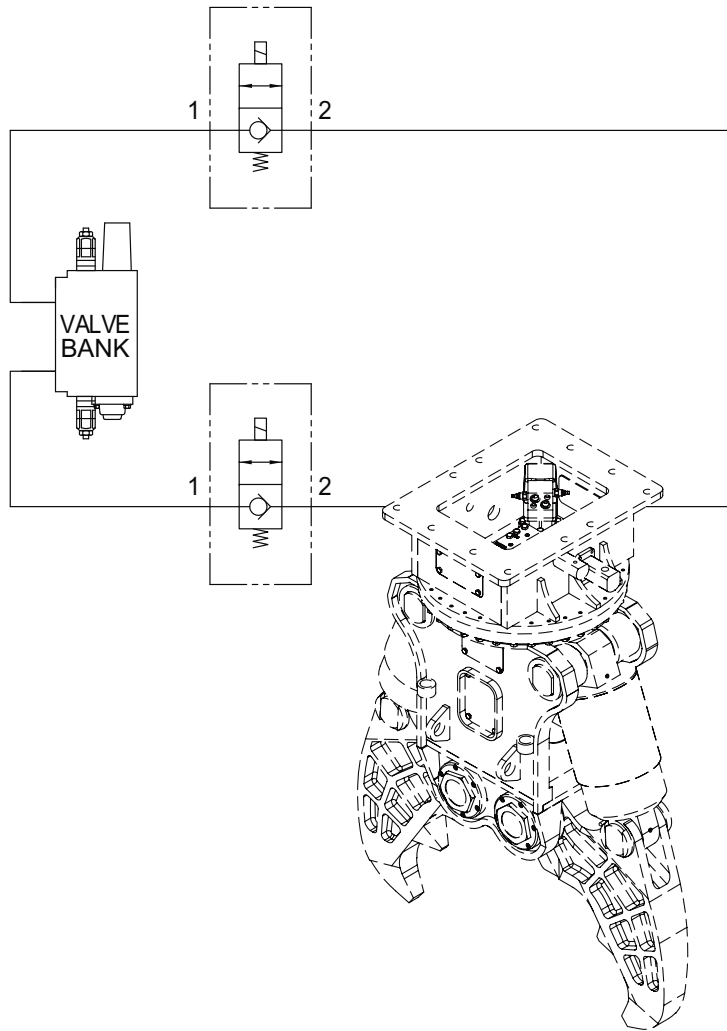
[ SHUT-OFF VALVE : CRUSHER/ GRAPPLE ]
