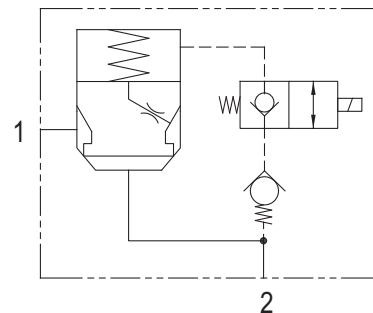
[ Hydraulic Schematic : NC ]
