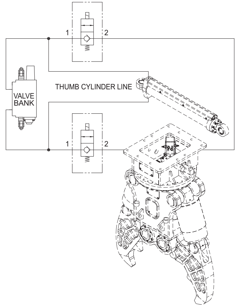
[ SHUT-OFF VALVE : THUMB/ CRUSHER COMBO ]
